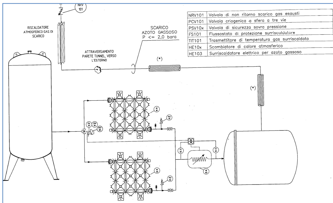
Fig. 19: Layout of the regeneration and baking system. We note that two vaporizers are needed for each trap in order to get a continuous operation. They will exchange every 8-10 hours to get alternatively heated-up to eliminate the frost accumulated on the surface.
