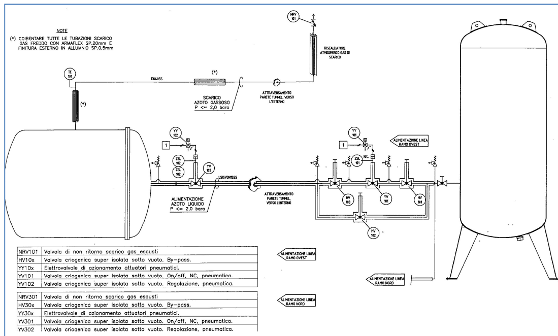
Fig. 18: LN2 transfer line - Central building
