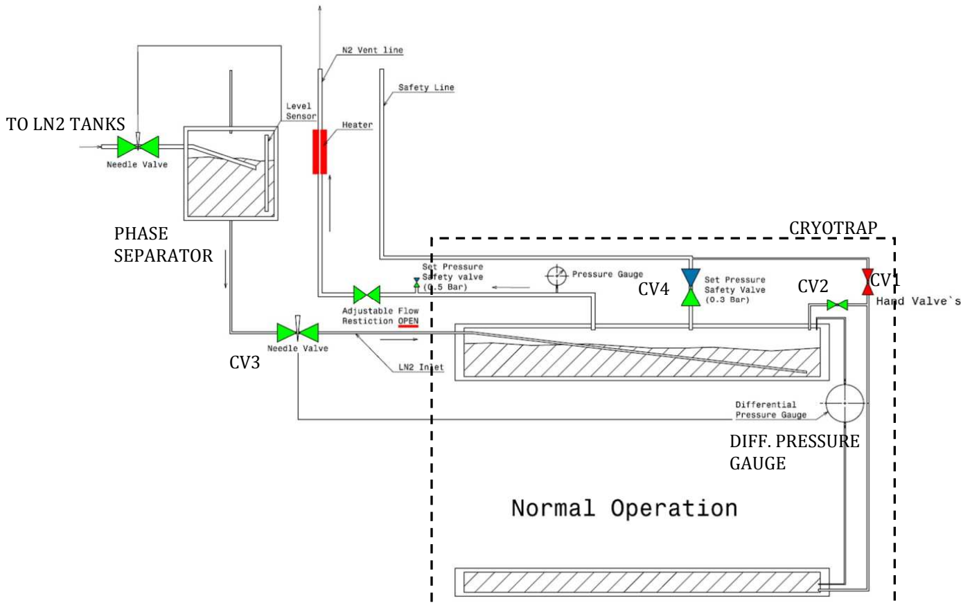
Figure 6: Schematic of the cryogenic controls during normal operation of the cryotrap (see also par 2.6 for a complete description of cryogenic piping equipment).
