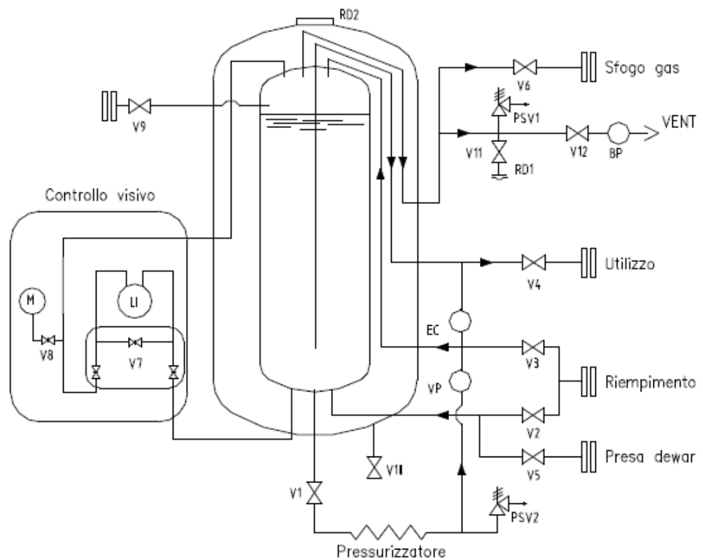
Fig. 17: Typical layout of the LN2 storage tank.
