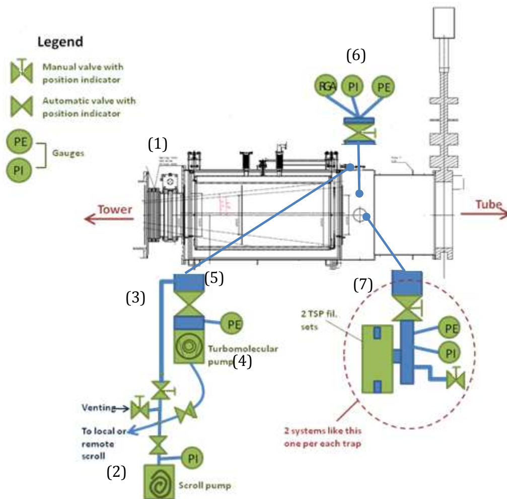
Fig 10 Sketch of the auxiliary vacuum system.
