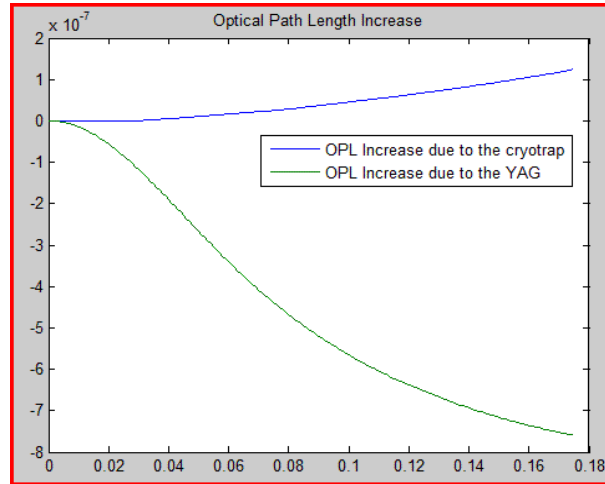
Fig. 13: Optical path length (OPL) increase due to thermal effects in the TM. The blue curve is the OPL increase due to the trap, while the green curve is the OPL increase due to the absorption of YAG power.
