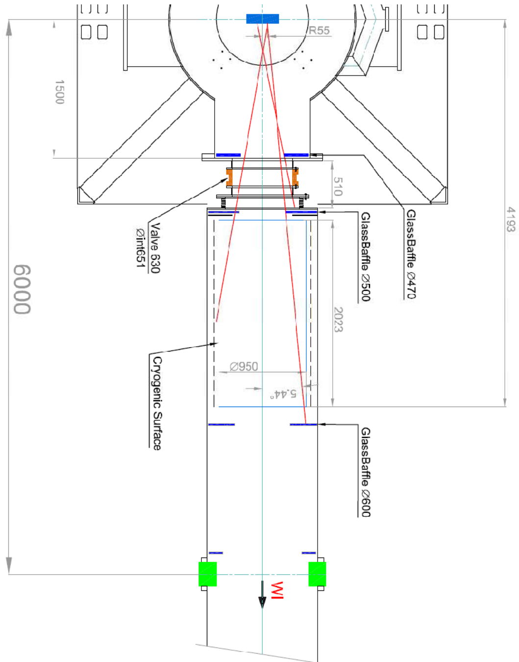
Fig. 11 Schematic of optical baffles setup around the cryotrap
