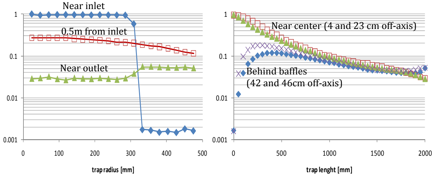
Fig 8. Normalized density of molecule tracks inside the trap along the trap radius at different length positions (left) and along the trap length at different distance from trap axis (right). The ratio between outlet and inlet values shows the escaped molecules fraction, about 0.03. (Molecules re-entered from the tube are not shown, to put in evidence the trapping effect). Baffles (aperture radius=300mm) installed at trap extremities affect the molecule distribution.
