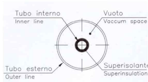
Fig. 18: Cross-sectional layout of the LN2 transfer line.
