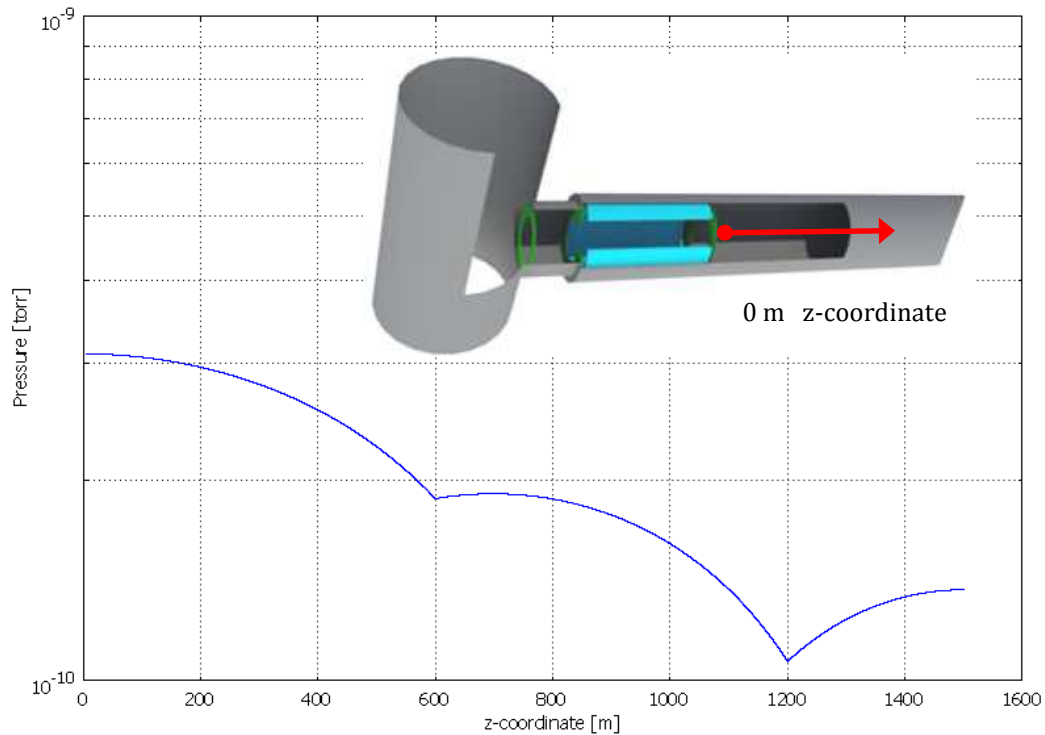
Fig. 7 Water pressure profile along the 3km tube calculated for the selected trap geometry
