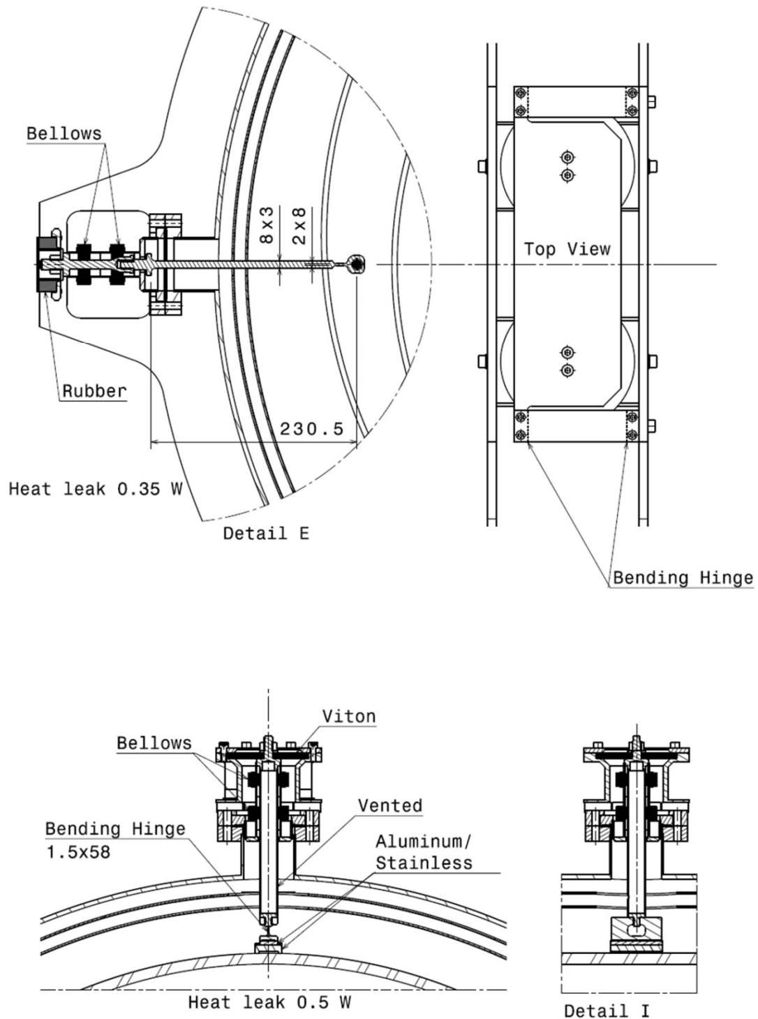
Fig. 15: Suspension system for the cryotrap.
