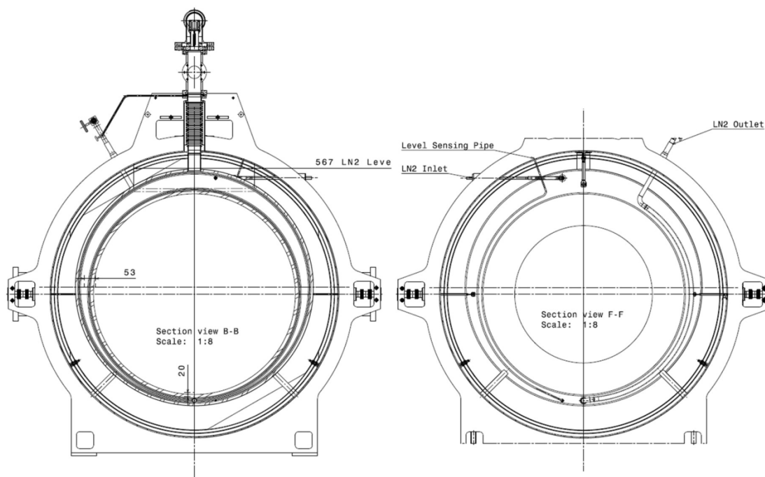
Fig. 5: Cross section of the cryotrap. The outer wall of the cryostat vessel is placed off-axis with respect to the vacuum vessel. The inner wall of the cryostat is placed on-axis
