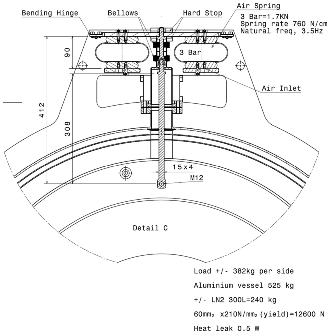
Fig. 14: The cold vessel of the cryotrap is suspended with air springs in order to isolate Advanced Virgo from possible bubbling noise produced by the cold vessel itself.
