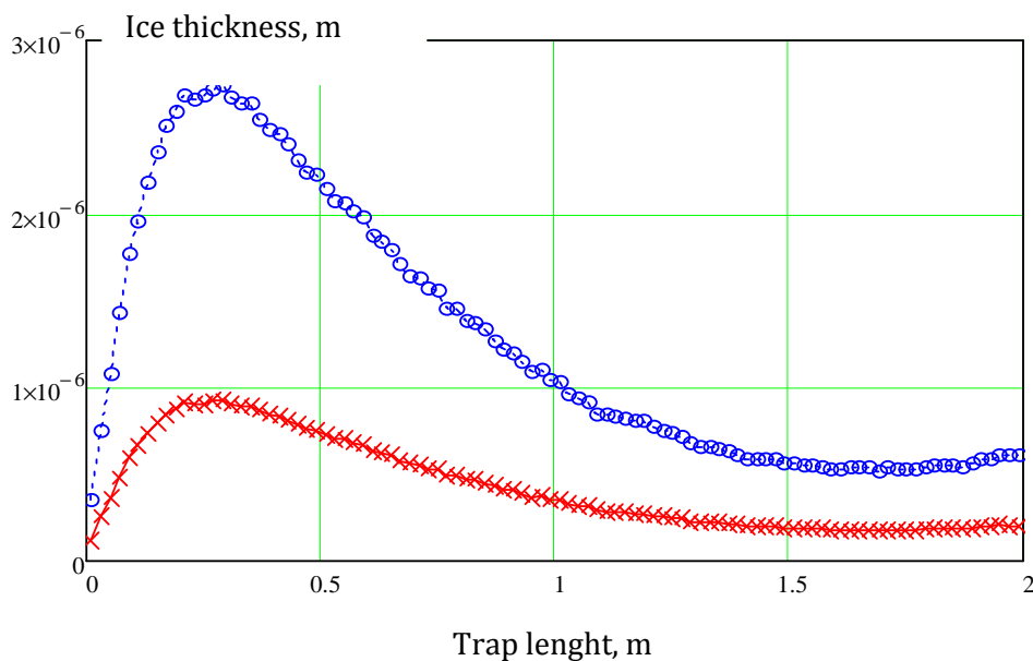
Fig.9. evaluation of the water deposit developed inside a trap after 1 year of service. Red curve='run' conditions (~2g of condensed water); blue curve= commissioning with very frequent tower openings (~6 g, considering venting every 2 months)
