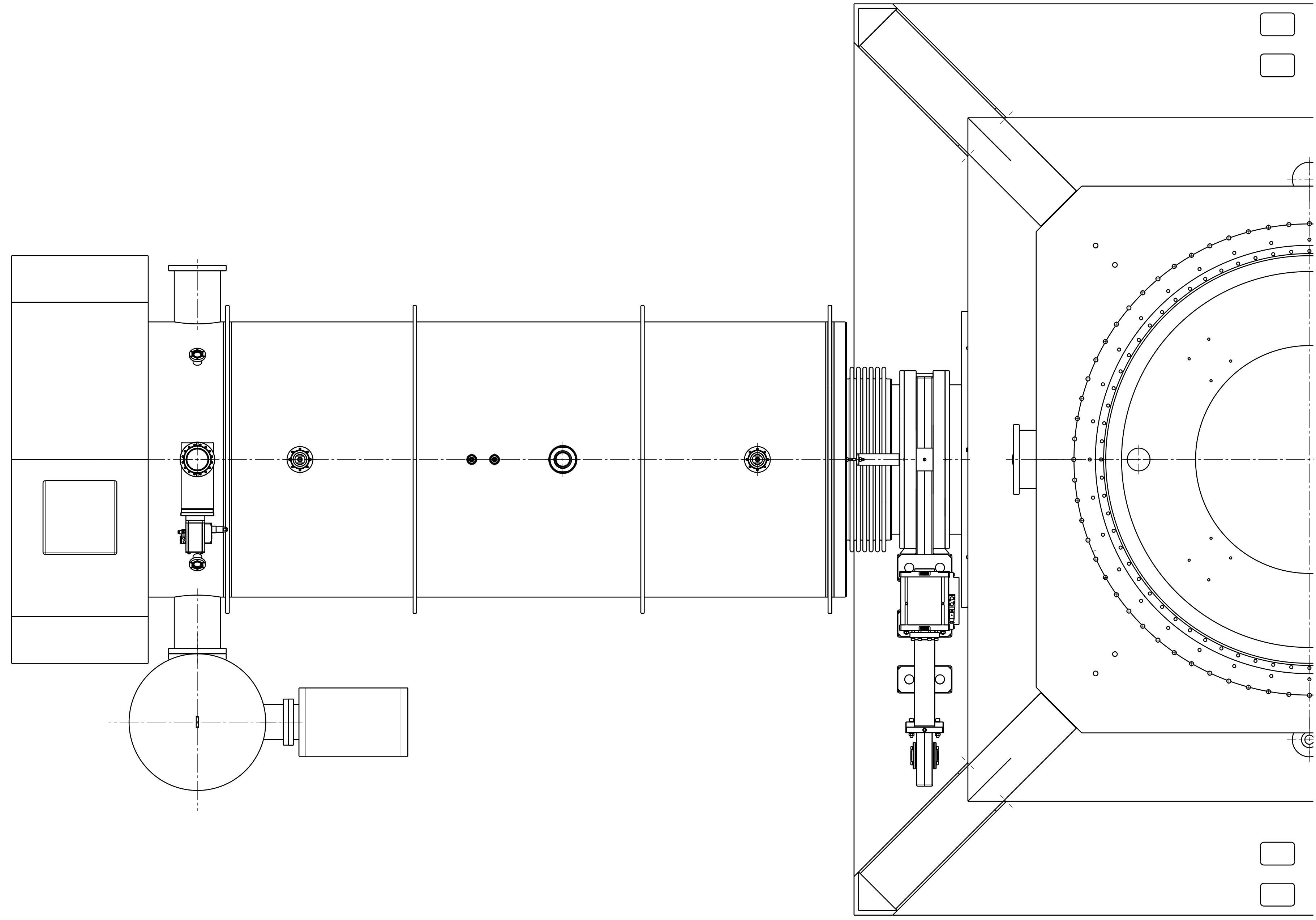
Auxiliary view A Scale: 1:12
