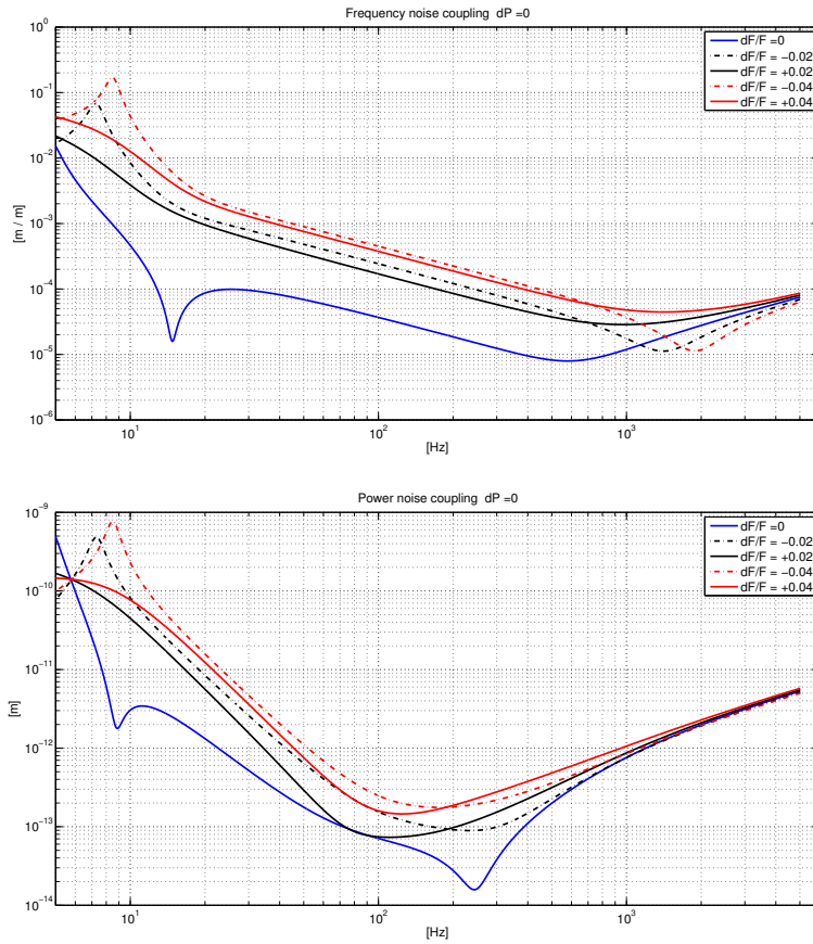
Figure 1.5: Dual recycled at full power configuration. Transfer functions in case of equal round trip losses ( RTL = 75 ppm) as a function of finesse asymmetry. Average finesse is 450. Top: frequency noise transfer function. Bottom: power noise transfer function.
