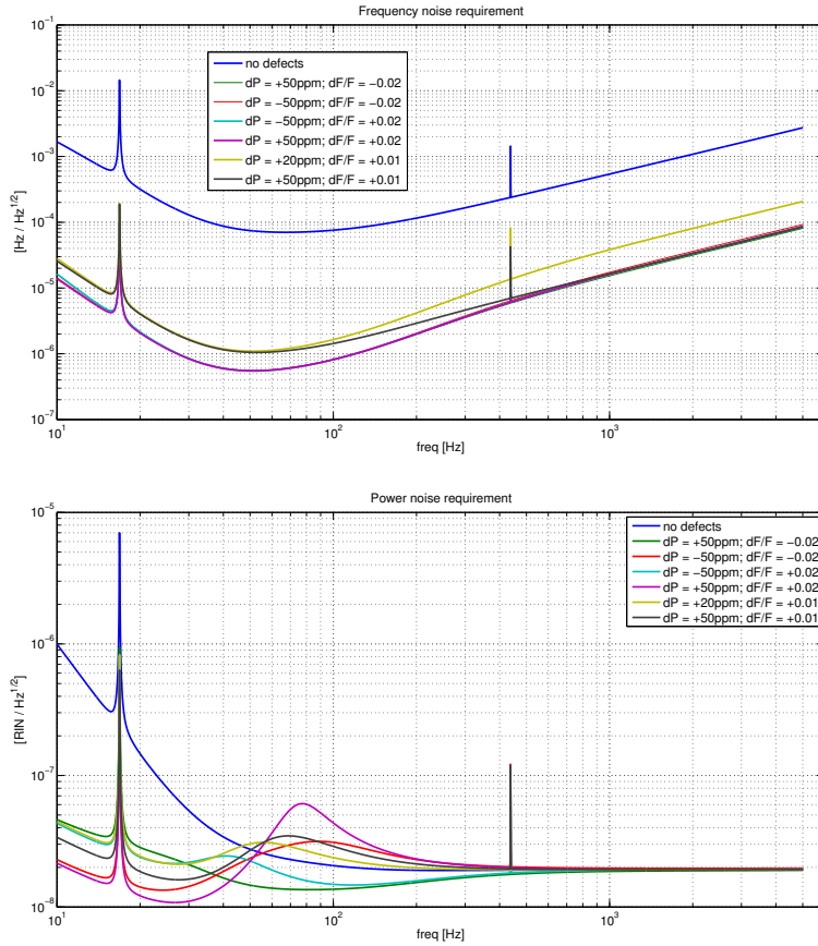
Figure 1.7: Technical noises requirements for power recycled at 25 W configuration, a safety factor of ten has been used to draw the requirements from nominal sensitivity. Different values of finesse and loss asymmetries have been used. Top: laser frequency noise at interferometer input. Bottom: laser intensity noise at interferometer input.
