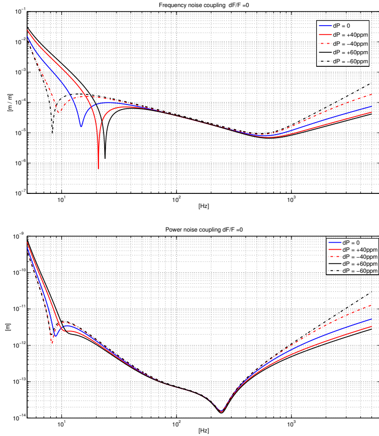
Figure 1.4: Dual recycled at full power configuration. Transfer functions in case of equal finesse ( F = 450 ) as a function of round trip loss asymmetry. Average round trip losses are 75 ppm. Top: frequency noise transfer function. Bottom: power noise transfer function.
