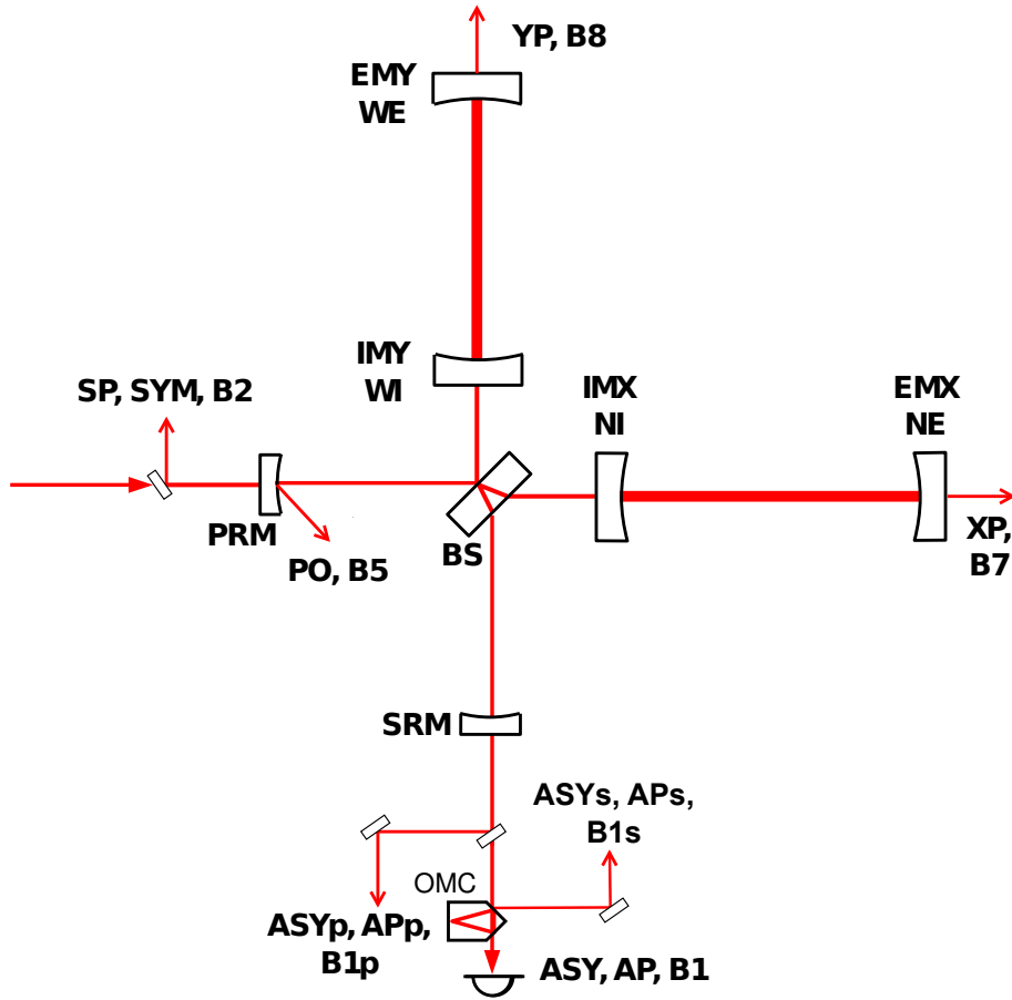
Figure 1.1: Optical layout of the Advanced Virgo interferometer, with the different naming conventions used for mirrors and output ports.
