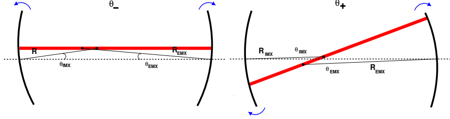
Figure 1.13: Effect of radiation pressure in a Fabry-Perot cavity. The two mirror modes become connected by an optical spring. The Fabry-Perot cavity mis-alignments can be described using the (+) plus and (-) minus modes. The combinations of single mirror mis-alignments giving the two modes depend on the cavity geometry.
