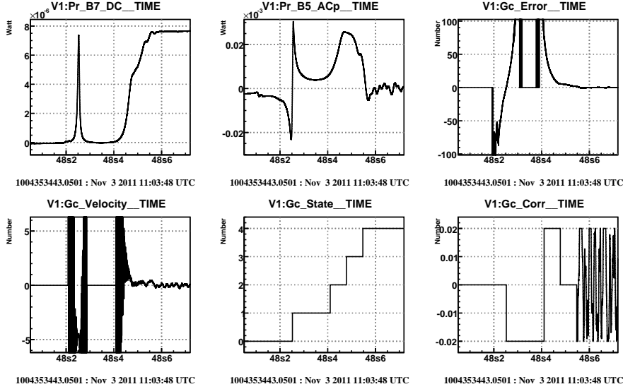
Figure 1.10: Experimental demonstration using Virgo+ of a lock with reduced force implemented in Gc. The error signal is calculated as B5\_ACp/B7\_DC and the velocity as the derivative of the error signal. Two pulses with opposite sign are applied. The lengths of the two pulses are calculated to bring the mirror back at resonance with velocity zero and are proportional to the velocity measured while crossing the resonance. The logic is implemented as a state-machine (0 = wait for resonance, 1 = first pulse, 2 = second pulse, 3 = wait for return to resonance, 4 = linear lock). The lock was acquired with a maximum correction of 0.02 Volt on 1 coil-pair, while a maximum of 0.8 Volt on 4 coil-pairs is available.
