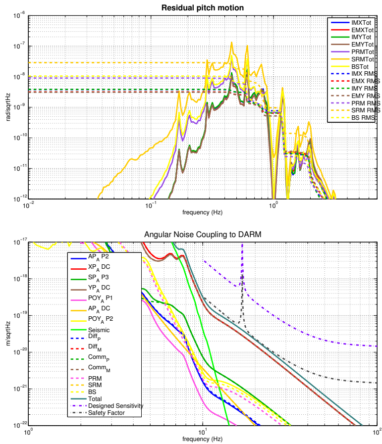
Figure 1.16: Mirror residual displacement and Automatic Alignment control noise projection for the low power interferometer with SRC on the top and on the bottom plot respectively. The control noise results to be compliant with the sensitivity requirements.
