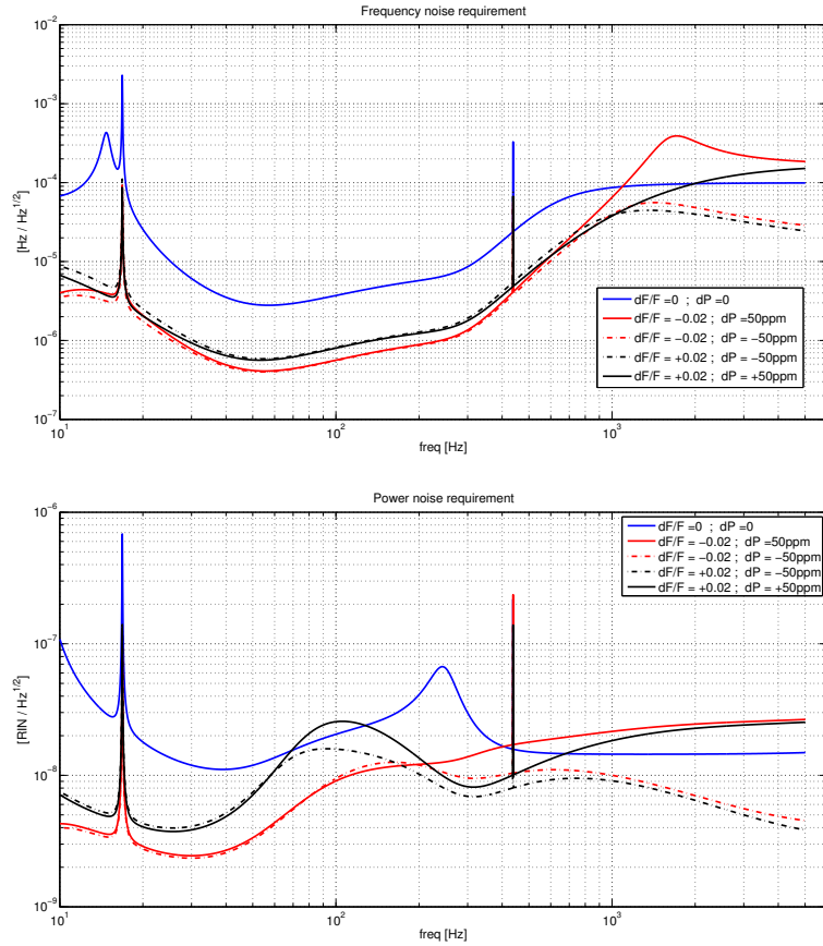
Figure 1.6: Dual recycled at full power configuration, technical noises requirements with a safety factor of ten used to draw the requirements from nominal sensitivity. Different values of finesse and loss asymmetries are used. Top: laser frequency noise at interferometer input. Bottom: laser intensity noise at the interferometer input. Blue curve: no defects. Red curves: dF/F = -2\% ; black curves: dF/F = +2\% . Solid curves: dP = +50 ppm, dashed curves: dP = -50 ppm.
