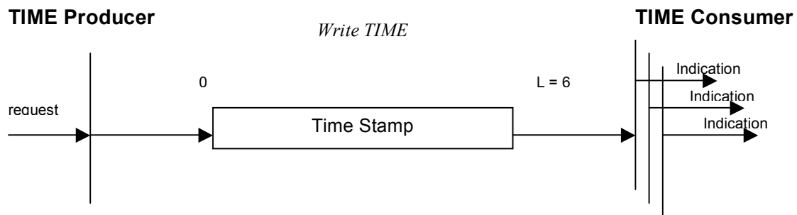
Figure 32: TIME Protocol
