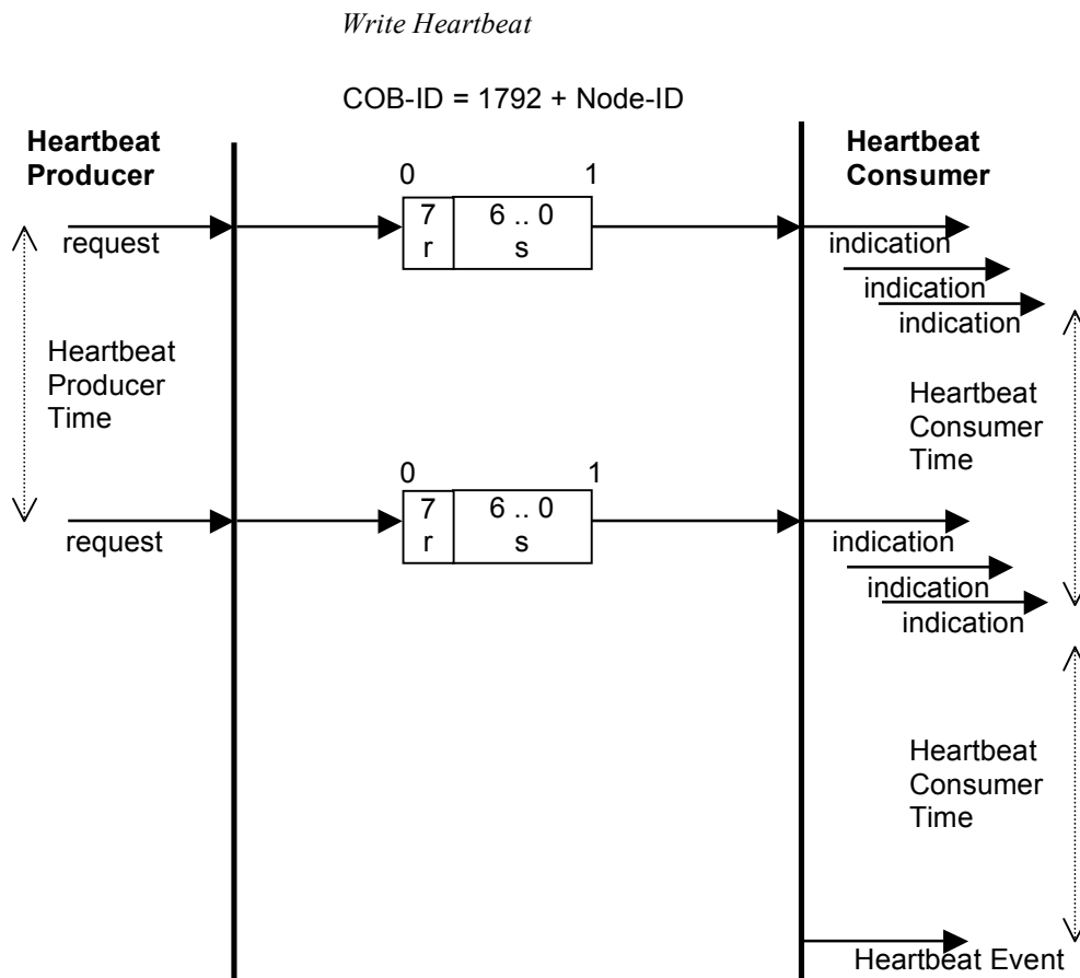
Figure 42: Heartbeat Protocol
