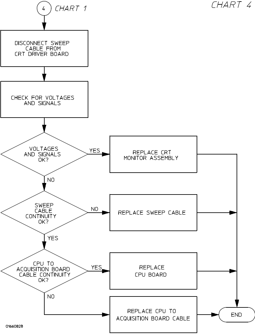
Troubleshooting Flowchart 4
