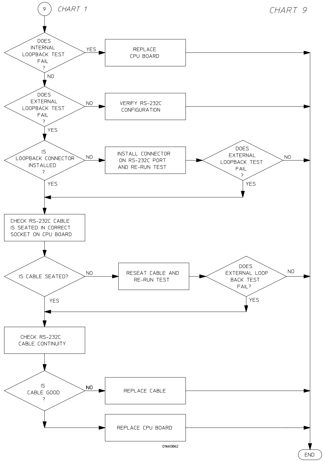
Troubleshooting Flowchart 9
